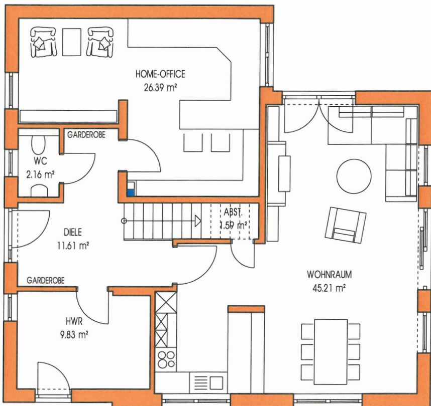
ERDGESCHOSS 1:75 VARIANTE HOMEOFFICE
